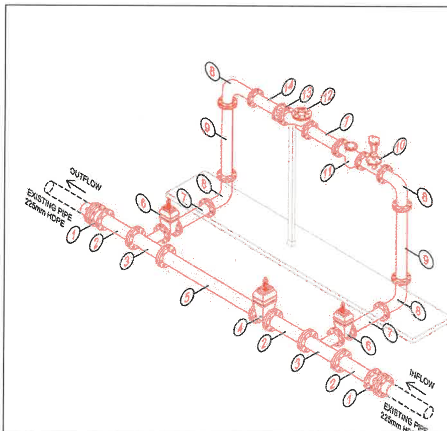
CONTOH PRESSURE REDUCING VALVE (PRV)
